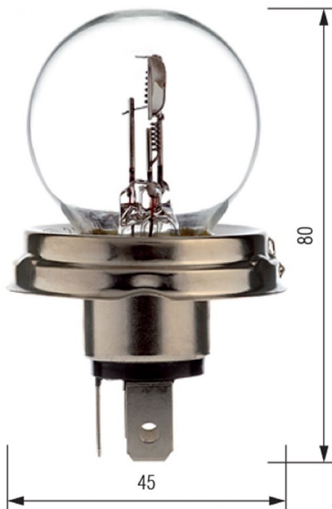
P45t 6V 45-40W Car
