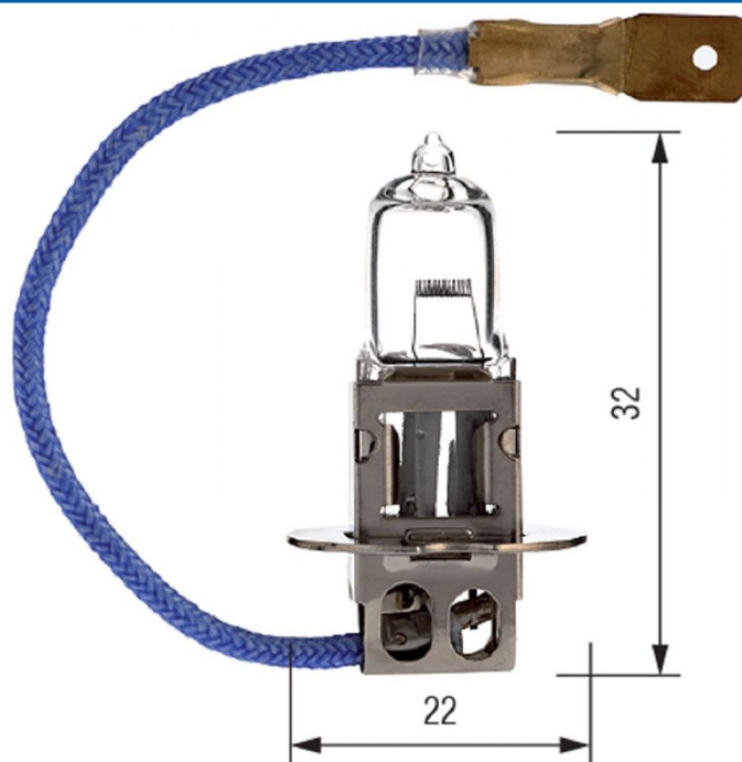
H3 PK22s 12V 130W RALLY Car
