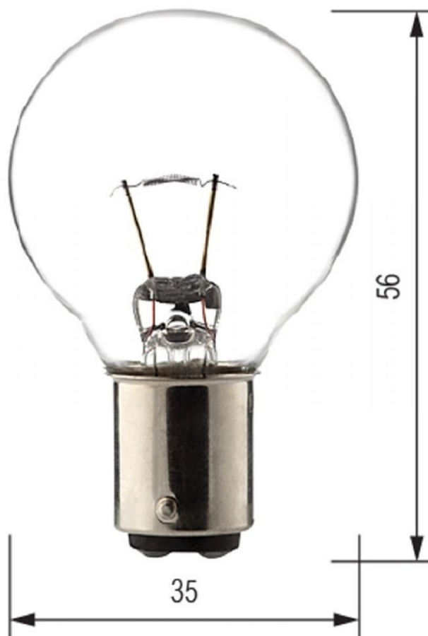
Ba15d 36x56 mm 24V 45W Car
