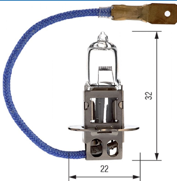
PK22s 11x42 mm 48V 45W Fork
