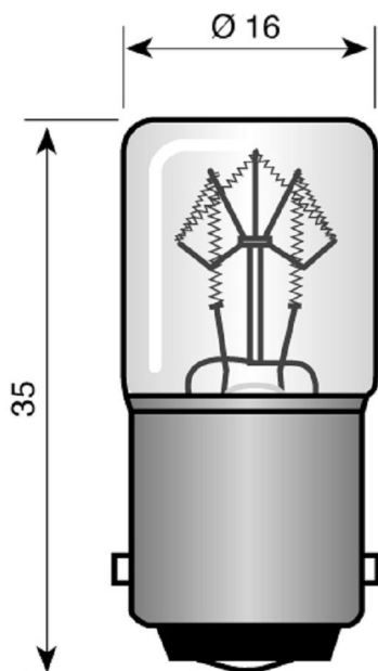
Ba15d 16x35 mm 60V 3W
