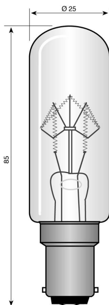
Ba15d 25x85 mm 130V 15W frosted
