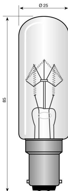
Ba15d 25x85 mm 130V 25W frosted
