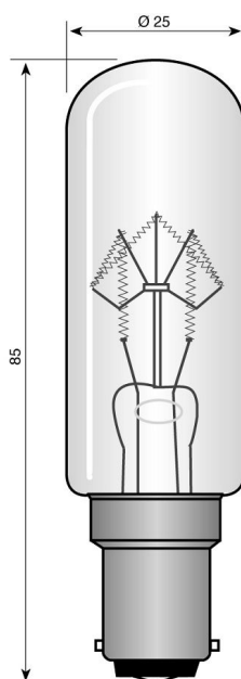
Ba15d 25x85 mm 230V 25W frosted
