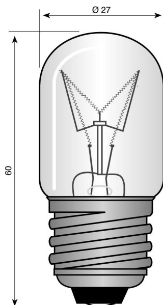
E27 27x 60 mm 36V 10W clear
