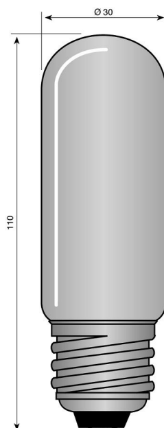
E27 28x110 mm 110V 40W frosted
