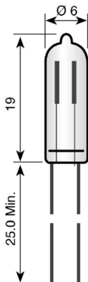
WE 6x19 mm 220-240V NEON clear RESISTOR
