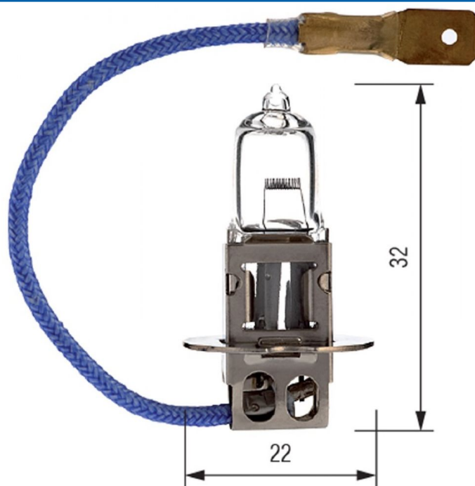
H3 6V 35W Car
