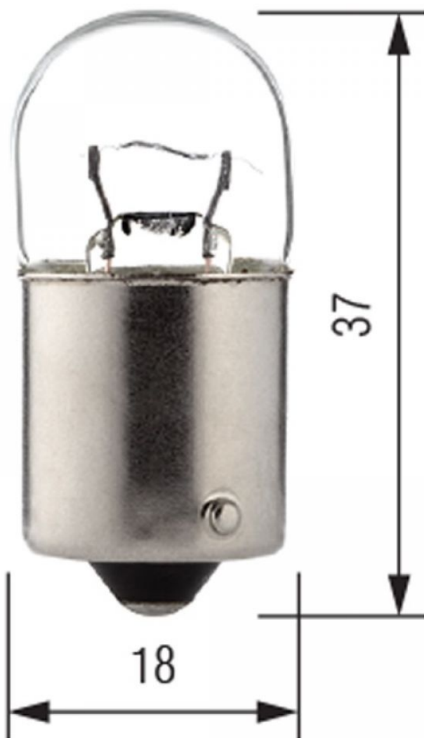
Ba15s 18x35 mm 48V 10W Fork
