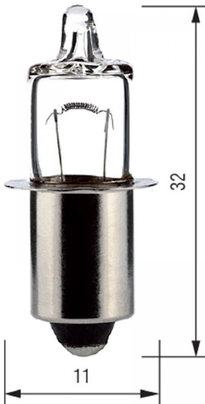
PX13.5s 9x30 mm 12V 15W Car
