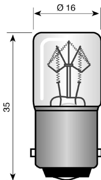
Ba15d 16x35 mm 48V 5W
