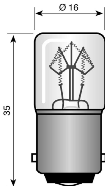
Ba15d 16x35 mm 220-260V 6-10W
